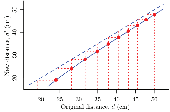
Fig. 5. Mapping from the original distance d to the new distance d' between the center of curvature of a moving robot, i , to a static robot, j . The red trajectory illustrates how, starting some value d_0 > R + r_i + r_j , d decreases stepwise until it becomes smaller than or equal to R + r_i + r_j . For the values used here, R + r_i + r_j corresponds to 21.85 cm. The value of d_0 used in this figure is 50 cm.
