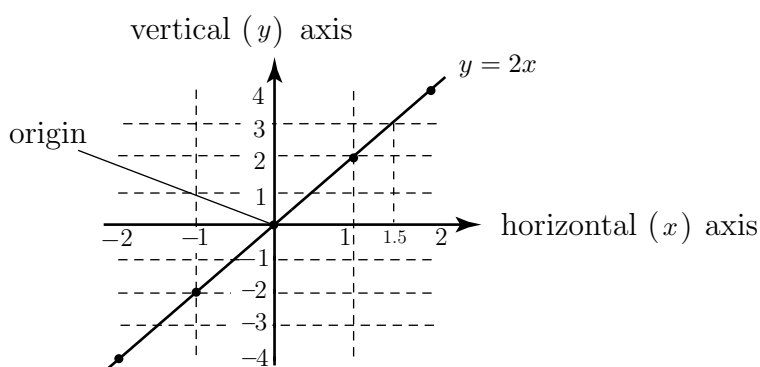
Figure 7: The two axes intersect at the origin
