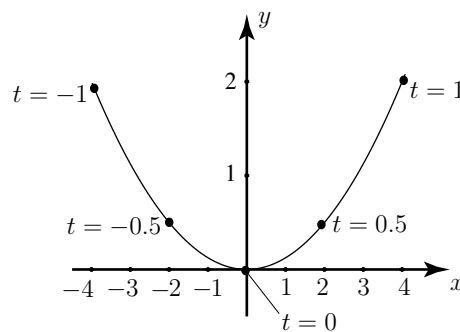
Figure 9: Graph of the function defined parametrically by x = 4t , y = 2t^2 , -1 \leq t \leq 1
