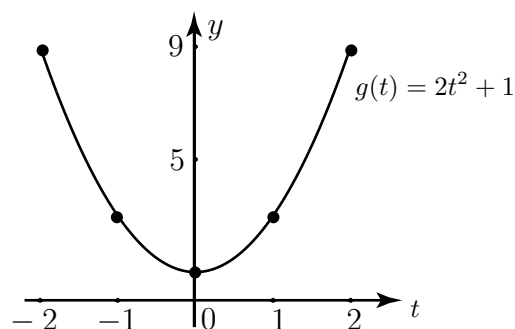
Figure 8: Graph of g(t) = 2t^2 + 1
