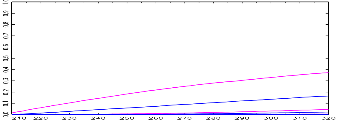
Figure 6: Rejection frequencies of A_{MAX}(10) and S_{MIN}(10, 2) for multiple bubble and crash episodes: \tau_{j,1} = 1
