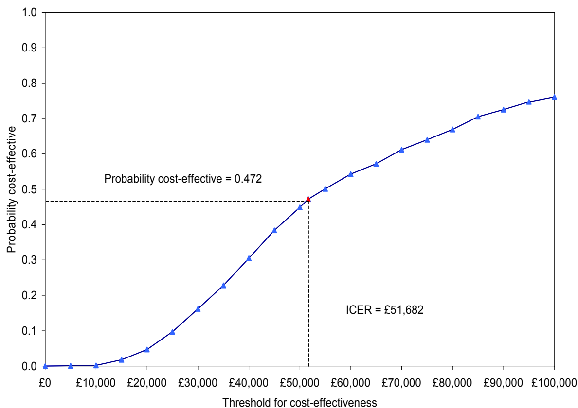
Figure 1.1: Cost-effectiveness acceptability curve example
